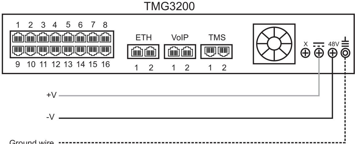
Figure 2.10 TMG3201 DC wiring diagram
