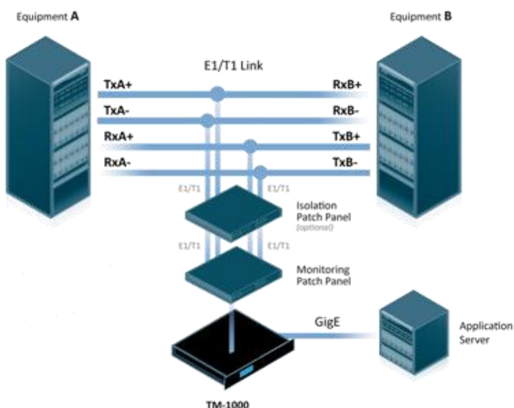
> Figure: sample integration of the Tmonitor TM2000
