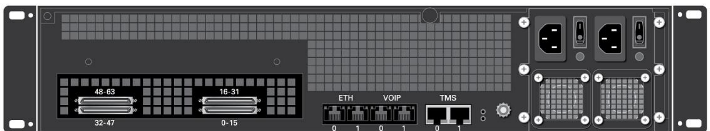
Tmedia TMG3200-TE, rear view AC (DC also available)
