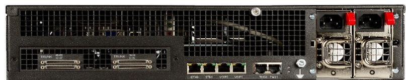
Tmedia TMG3200-TE 2U VoIP gateway (Back View)
