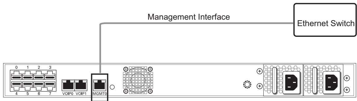
Management Interface
