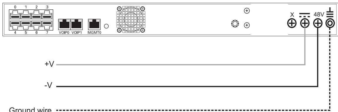
Figure 2.12 800 Series Unit DC Wiring Diagram
