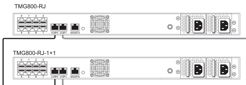
Figure 2.10 Connecting to the Tmedia Control Network
