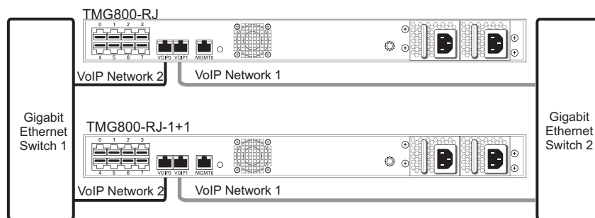
Figure 2.11 Connecting to the VoIP Network
