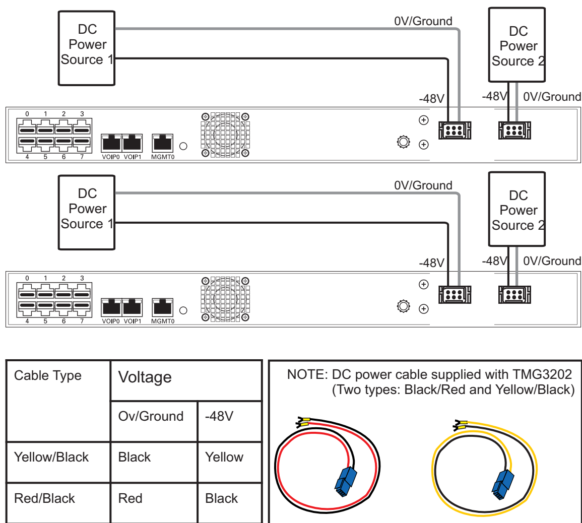
Figure 2.14 TMG800 and TMG800 +1 DC Power Connections
