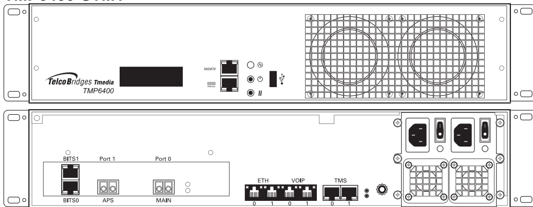
Figure 1.2 TMP6400 Telecom Units Front and Rear Views
