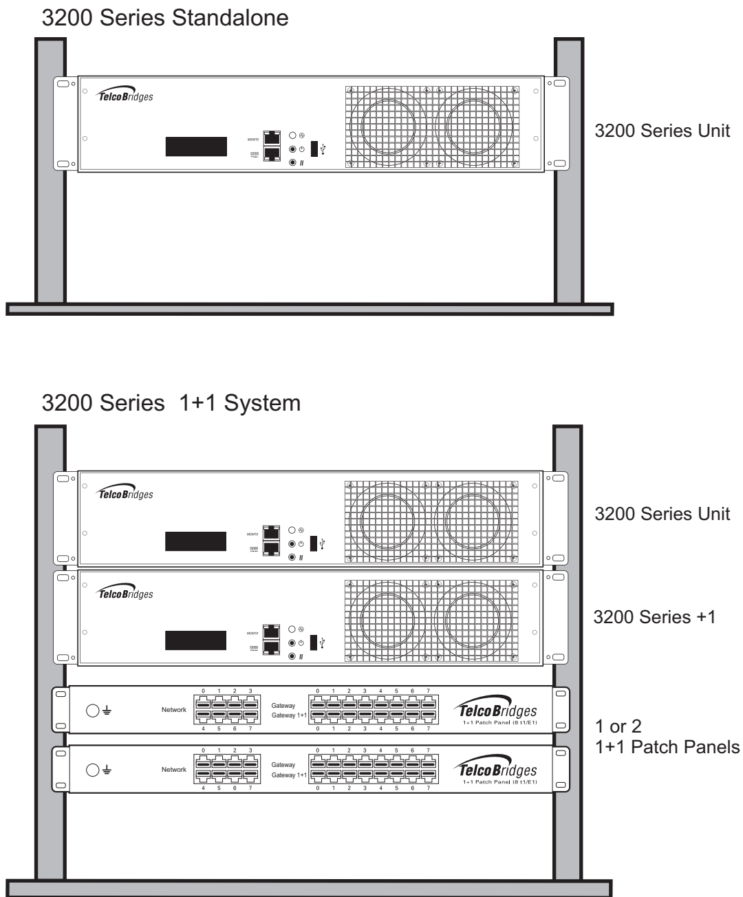
Figure 2.1 Rackmounting the Equipment
