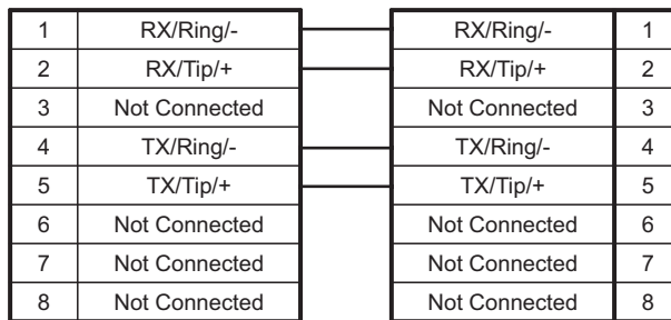
RJ48C (T1/E1) Wiring Schematic: Straight Cable
