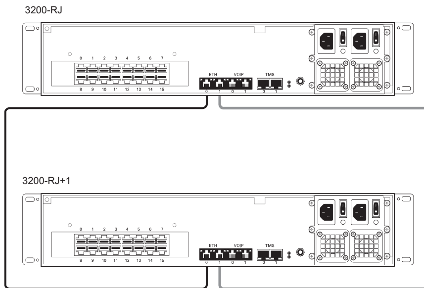
Figure 2.11 Connecting to the Control Network
