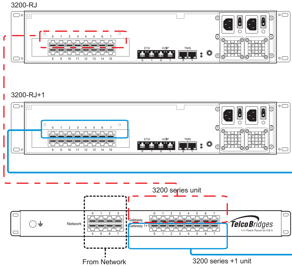
Figure 2.13 3200-RJ and 3200-RJ+1 connecting to the TDM 1+1 8/T1/E1 1+1 patch panel
