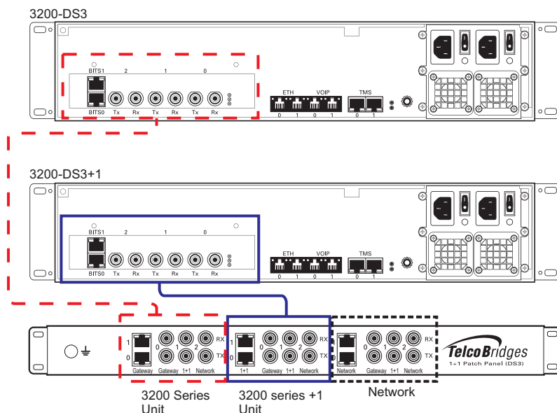
Figure 2.15 3200-DS3 and 3200-DS3+1 connecting to the TDM 1+1 DS3 1+1 patch panel
