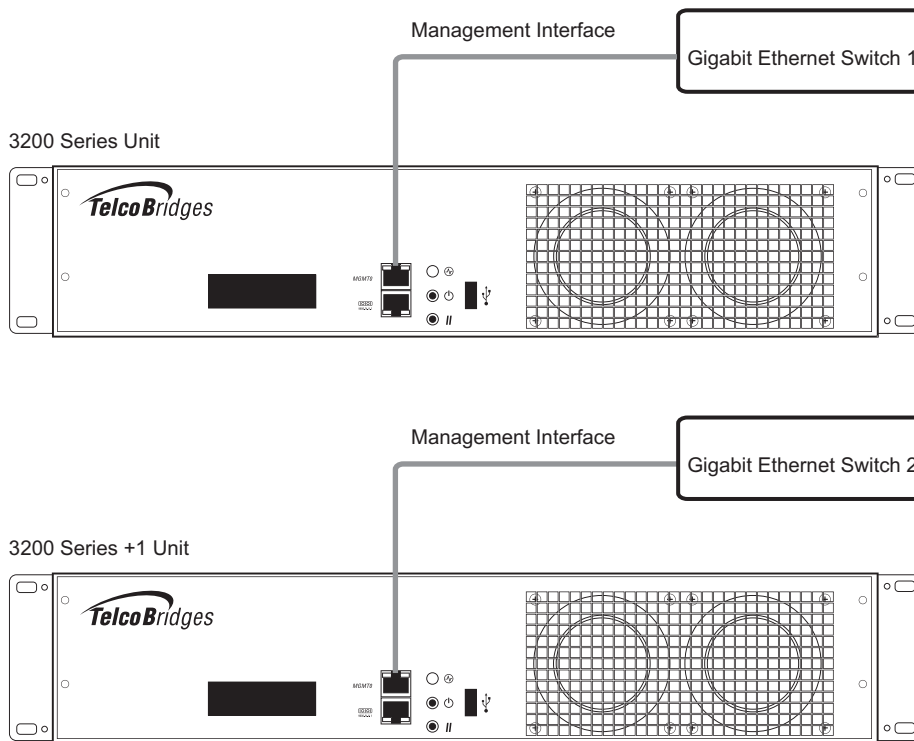
Figure 2.10 3200 Series 1+1 System Management Interface
