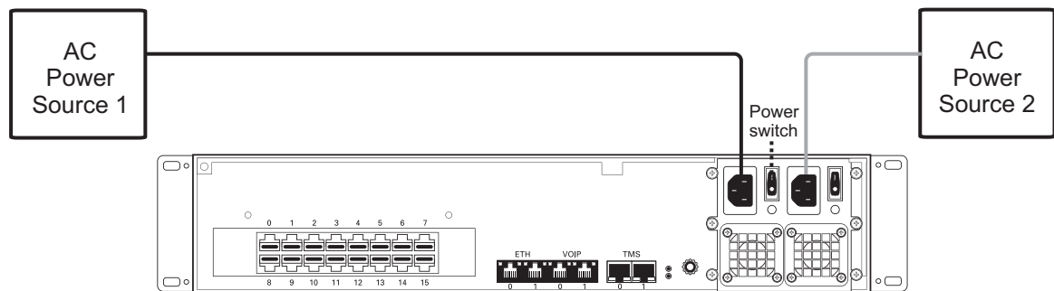
Figure 2.8 3200 Series Gateway AC Power Connection
