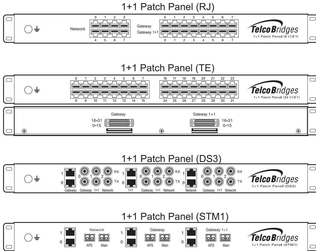
Figure 1.2 1+1 Patch Panels
