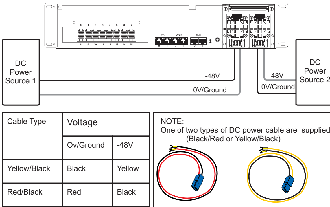
Figure 2.9 3200 Series Gateway DC Wiring Diagram
