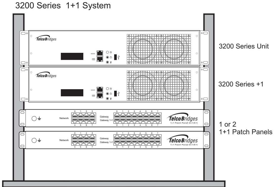
Figure 2.1 Rackmounting the Equipment
