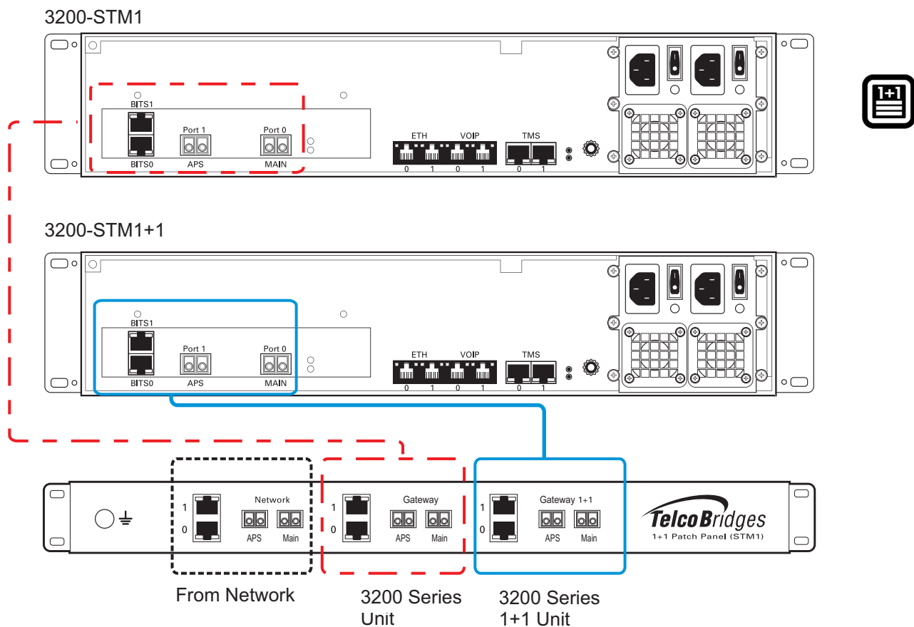
Figure 2.17 3200-STM1 and 3200-STM1 +1 connecting to the STM1 1+1 patch panel
