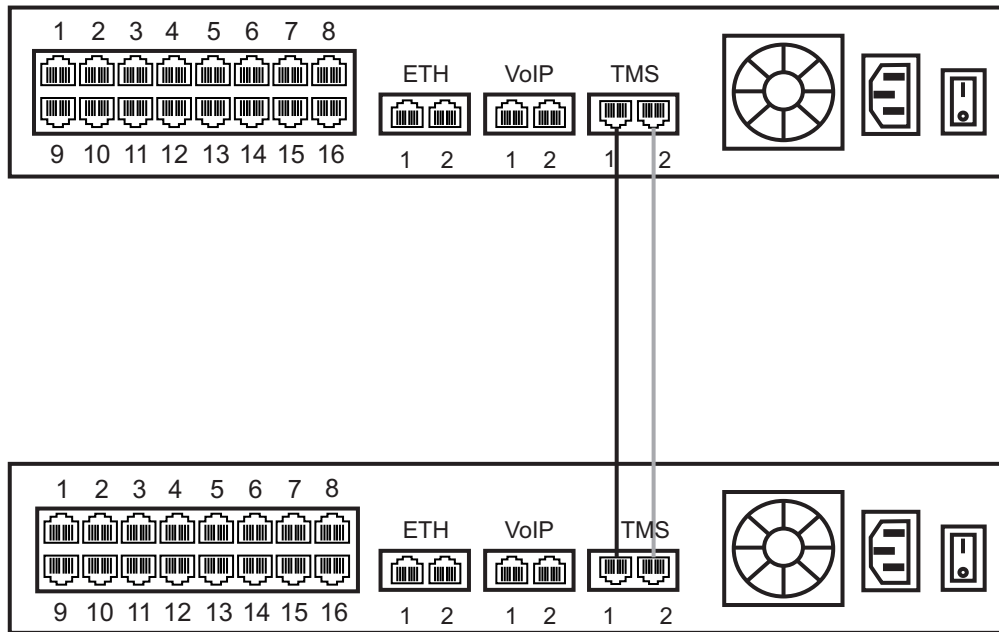
Figure 2.13 Interconnecting two TMP6400 units.
